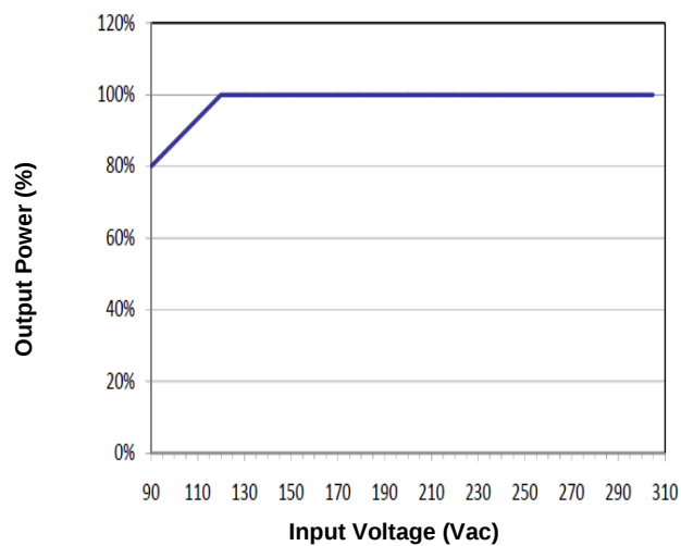
Figure 8: Output Power vs. Input Voltage
