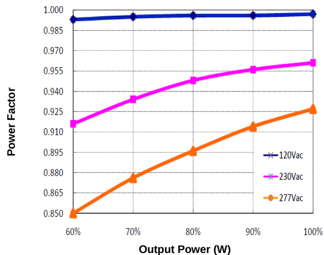
Figure 10: Power Factor vs. Output Power
