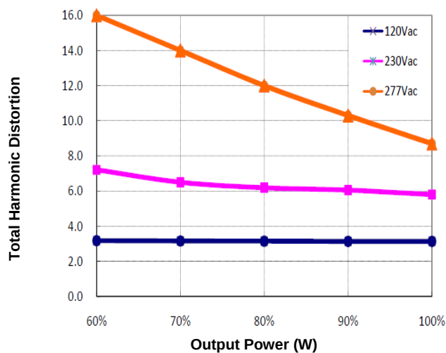
Figure 11: Total Harmonic Distortion vs. Output Power
