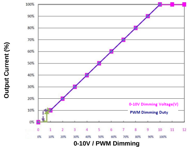
Figure 12: 0-10V/PWM Dimming Curve
