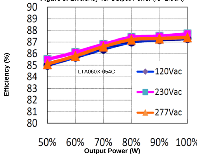
Figure 5: Efficiency vs. Output Power ( I_o=1.10A )
