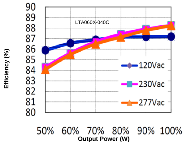
Figure 4: Efficiency vs. Output Power ( I_o=1.50A )
