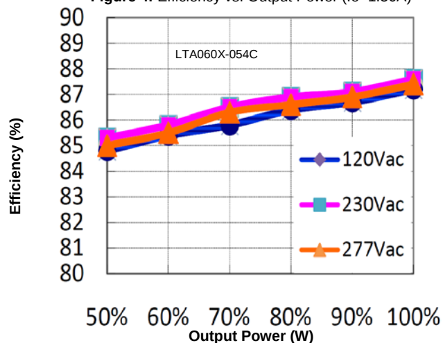
Figure 6: Efficiency vs. Output Power ( I_o=1.50A )
