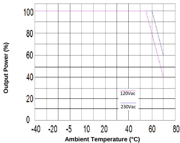
Figure 7: Output Power vs. Ambient Temperature
