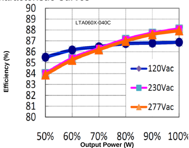
Figure 3: Efficiency vs. Output Power ( I_o=1.90A )
