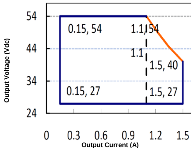
Figure 2: Typical V-I Characteristic Curve (LTA060X-054C)
