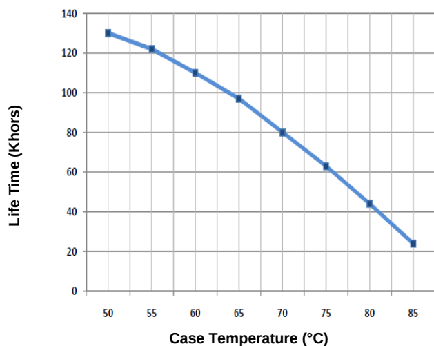
Figure 9: Life Time vs. Case Temperature
