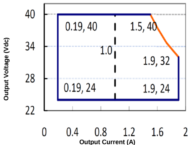
Figure 1: Typical V-I Characteristic Curve (LTA060X-040C)
